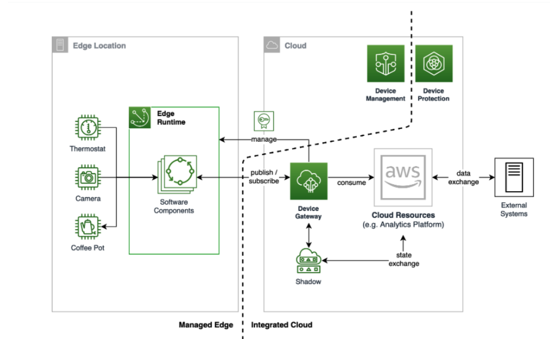
Figure 1. Generic architecture for sustainable IoT devices
